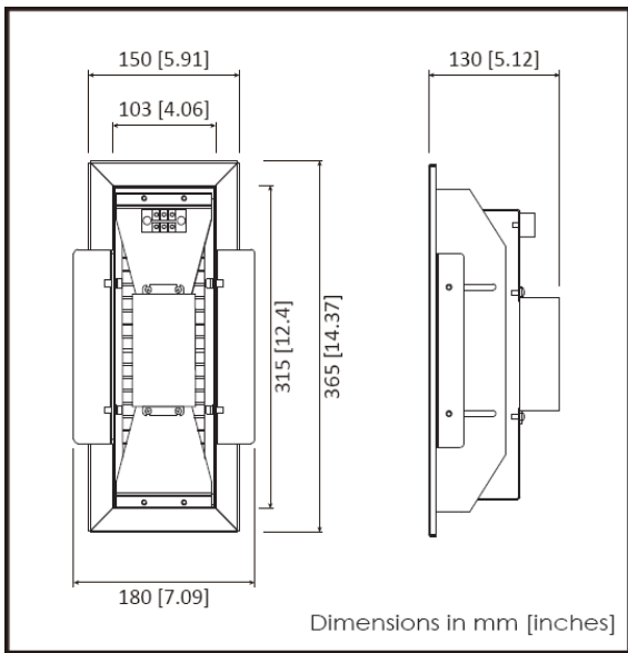
30 Watt High Powered Recessed LED Light
