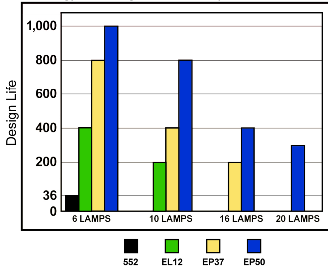
Technology vs. Design Life vs. Lamp Load
